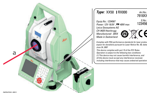
a) Laser beam
